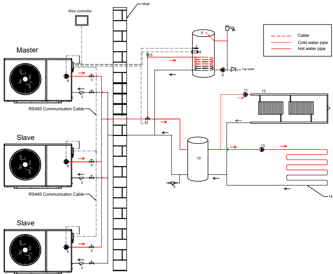
Heating&Cooling+Hot water Installation Instructions Schematic
